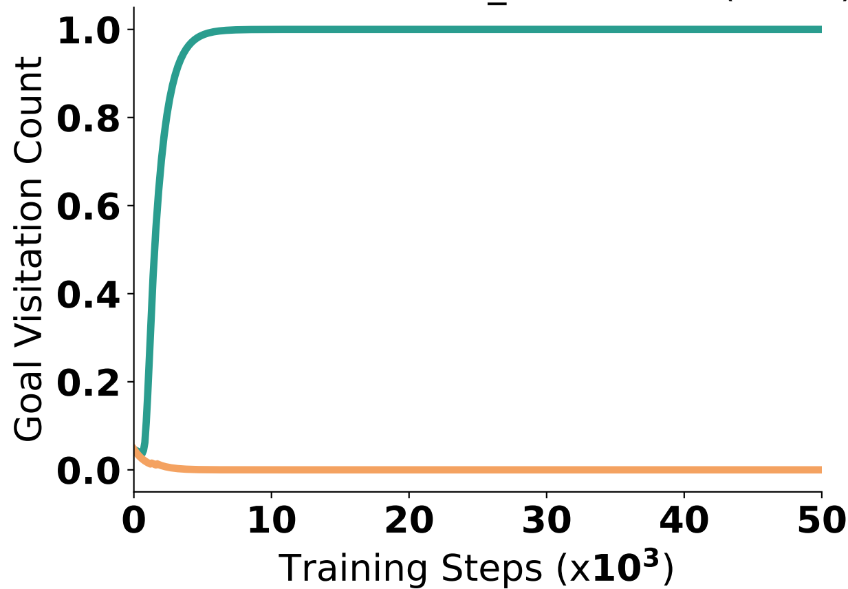
Gridworld-Bottleneck_FullRandom(100%)
